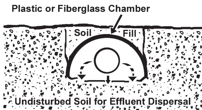
Figure 4. Soil infiltration chambers are sometimes used instead of gravel for effluent dispersal in absorption field trenches. This drawing represents one of several chamber designs available from commercial suppliers.
